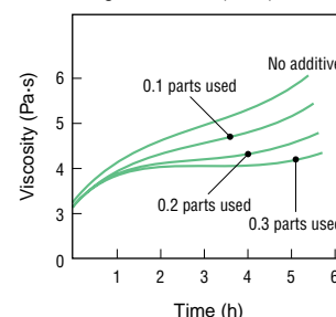
KE-1212 (A/B/C): Addition cure type Control Agent No. 6-10 (20°C)
